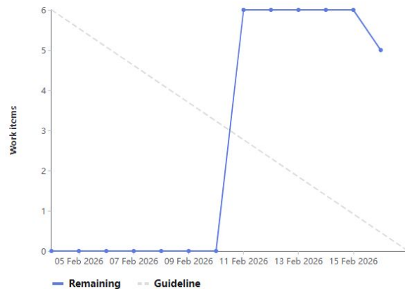
Burndown chart
