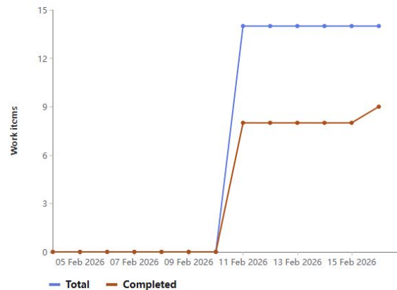
Burnup chart
